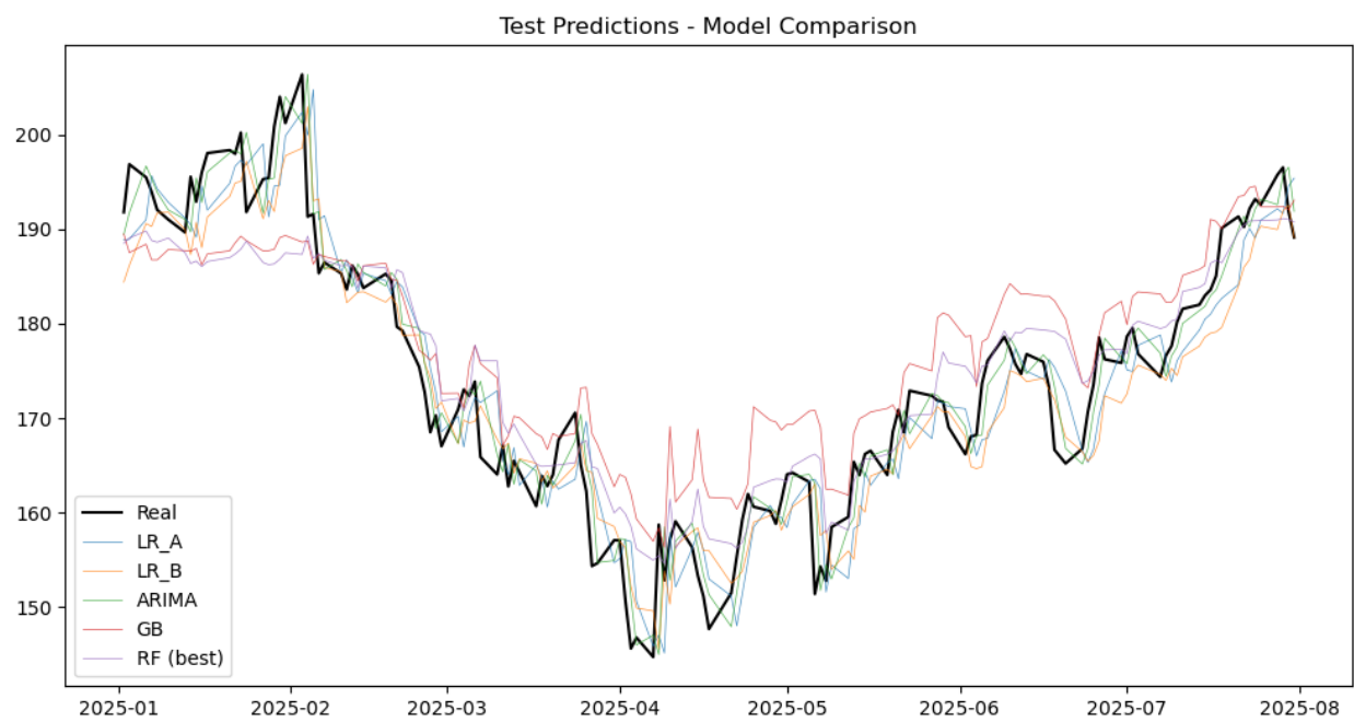
Figure 12. Test Predictions – Model Comparison
