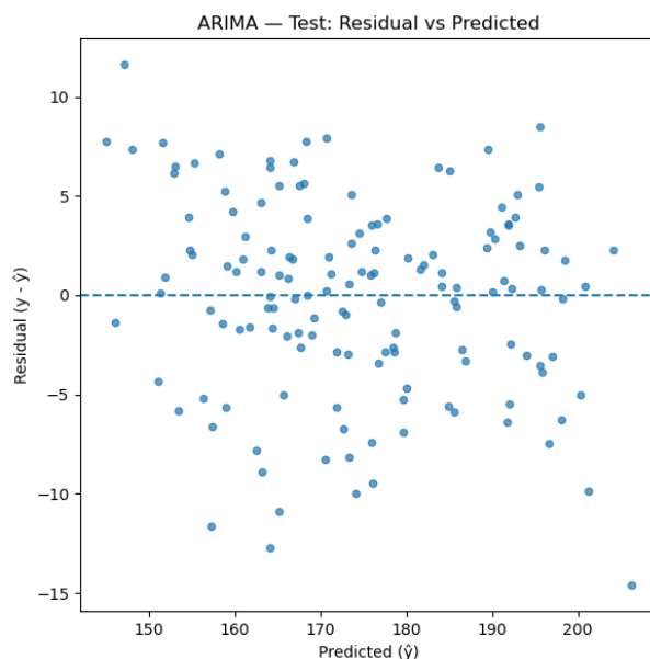
Figure 13. Residuals vs Predicted: ARIMA Test
